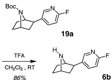
Scheme 4. Synthesis of norchlorofluorepibatidine ( 6b ).
