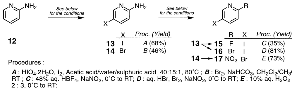
Scheme 2. Synthesis of 2-fluoro-5-iodopyridine (15), 2-bromo-5-iodopyridine (16), and 5-bromo-2-nitropyridine (17).
