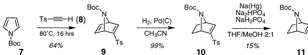
Scheme 1. Synthesis of 7- tert -butoxycarbonyl-7-azabicyclo[2.2.1]hept-2-ene (11).
