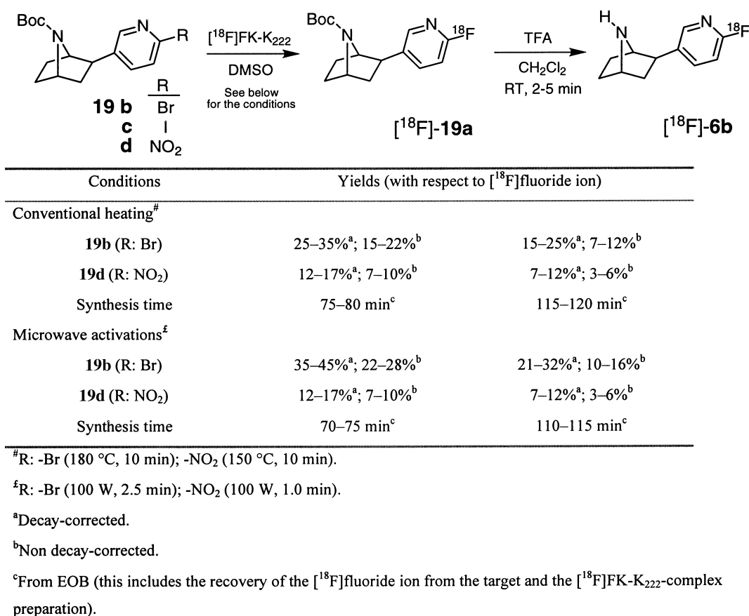
Scheme 5. Radiosynthesis of N -Boc protected [ 18 F]norchlorofluoroepibatidine ([ 18 F]- 19a ) and [ 18 F]norchlorofluoroepibatidine ([ 18 F]- 6b ); Conditions and yields.
