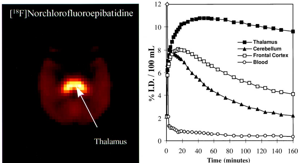
Figure 4. Baboon ( Papio papio ) brain PET images and time-activity curves for selected brain areas and blood following iv injection of [ ^{18}\text{F} ]nor-chlorofluoroepibatidine ([ ^{18}\text{F} ]-6b).
