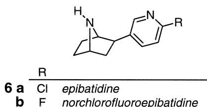
Figure 2. Chemical structure of epibatidine ( 6a ) and norchloro-fluoroepibatidine ( 6b ).
