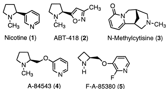
Figure 1. Chemical structure of nicotine (1), ABT-418 (2), N -methylcytisine (3), A-84543 (4), and F-A-85380 (5).
