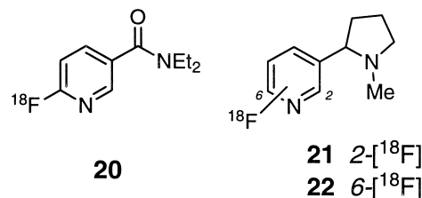
Figure 3. Chemical structure of 6-[ ^{18}\text{F} ]fluoronicotinic acid diethylamide ( 20 ) and 2- and 6-[ ^{18}\text{F} ]fluoronicotine ( 21 and 22 ).
