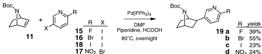
Scheme 3. Synthesis of epibatidine analogues 19a–d by reductive palladium-catalyzed Heck-type coupling.
